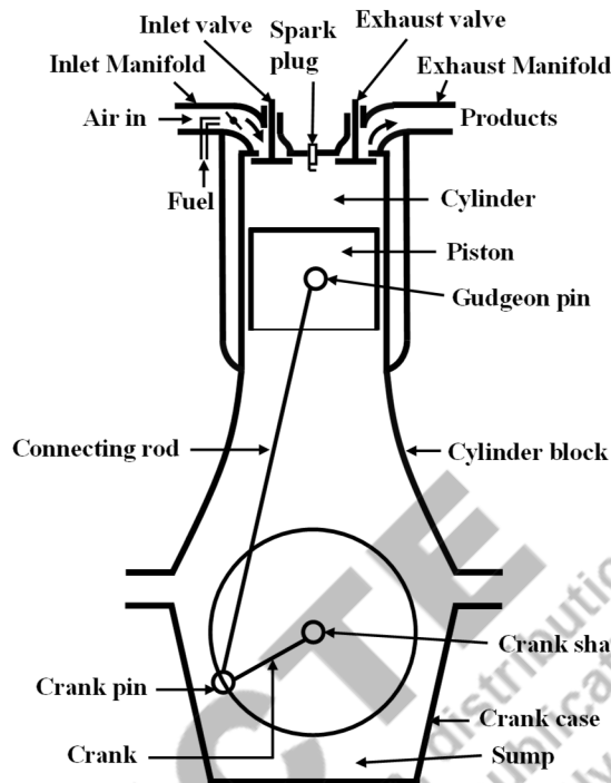
Figure 2.5: A schematic of different parts typically present in an SI engine
