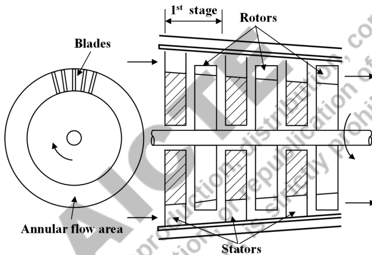
Figure 5.10: Schematic of an axial-flow compressor
