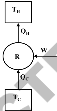
Figure 5.11: Schematic of energy transfers in a refrigeration system
